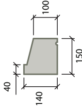
Slip Cill CL10 Weight: 39.4kg/m
