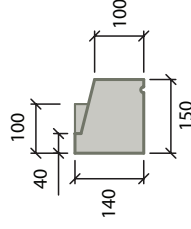
Stooled Cill CL11 Weight: 39.4kg/m Also available with 140mm stools - ref CL12
