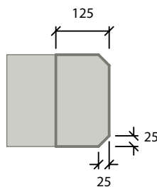
Chamfered Quoin MA09 Weight: 25.9kg
